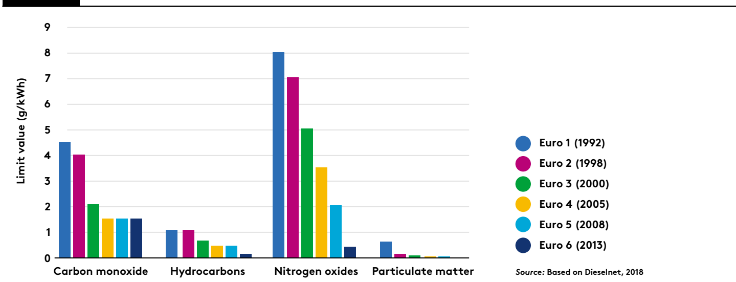
Figure 5.2 Maximum levels of exhaust pipe emissions allowed at each EU standard for HGVs
